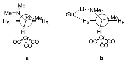
Figure 2. (a) Average solution-state conformation of the benzylic side chain of [ (R) - N,N -dimethyl-1-phenylethylamine]Cr(CO) 3 ] as inferred from NOEDS. (b) Newman projection of the possible directed orthometallation intermediate along the C α -C ipso bond.
