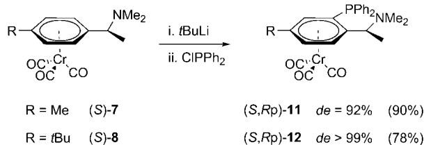
Scheme 4. Products obtained in the ortho -functionalisation of ( S )- 7 and ( S )- 8 .
