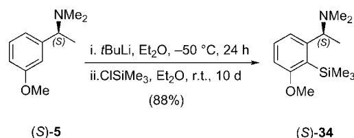
Scheme 12. Synthesis of ( S )- 34 .
