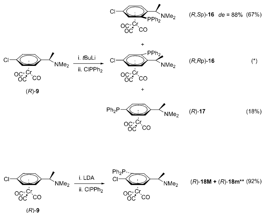
Scheme 6. Products obtained in the ortho -functionalisation of ( R )- 9 . Yields of isolated products are reported in parentheses. * See Table 2. ** This notation indicates the two regioisomeric products bearing a diphenylphosphanyl group ortho to the Cl substituent whose absolute configuration could not be assigned.
