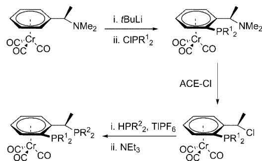
Scheme 1. General synthetic strategy for the preparation of “Daniphos”-like diphosphanes. ACE-Cl = 1-chloroethyl chloroformate.
