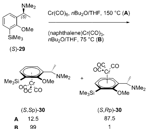
Scheme 9. Relative amounts of diastereomeric complexes obtained in the complexation of ( S )- 29 under thermodynamic (A) and kinetic (B) conditions.
