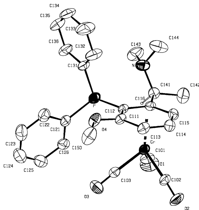
Figure 12. Displacement ellipsoids plot (PLATON) of (S,Sp)\text{-40} . Ellipsoids are shown at the 30% probability level. The H-atom attached to the stereogenic centre is shown with arbitrary radius; other H-atoms have been omitted for clarity.
