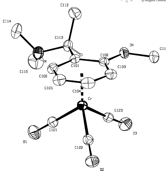
Figure 4. Displacement ellipsoids plot (PLATON) of ( S,Sp )- 28 . Ellipsoids are shown at the 30% probability level. The H-atom attached to the stereogenic centre is shown with arbitrary radius; other H-atoms have been omitted for clarity.
