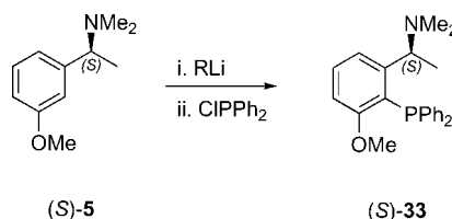
Scheme 11. Lithiation and subsequent electrophilic quenching of ( S )- 5 .
