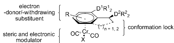
Scheme 2. Accessibility of a modular ligand architecture based on [(\eta^6\text{-arene})\text{Cr}(\text{CO})_3] complexes.
