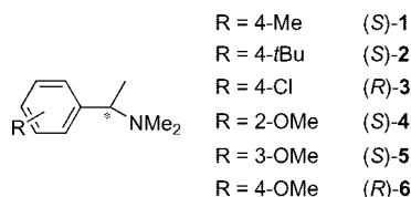
Figure 1. Phenylethylamines which have been complexed to the \text{Cr}(\text{CO})_3 moiety to synthesise the “Daniphos” ligands reported in this paper.
