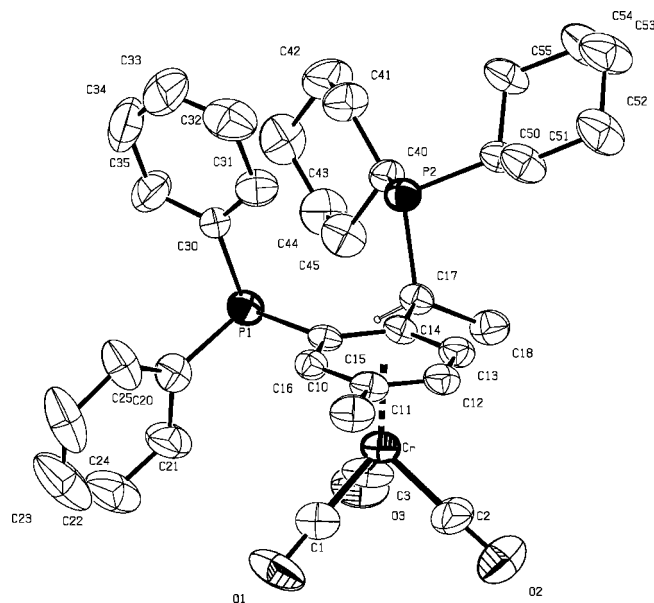
Figure 3. Displacement ellipsoid plot (PLATON) of ( S,Rp )-23b. Ellipsoids are shown at the 30% probability level. The H-atom attached to the stereogenic centre is shown with arbitrary radius; other H-atoms have been omitted for clarity.
