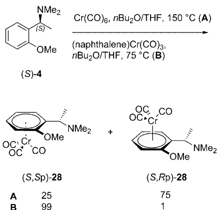
Scheme 8. Relative amounts of diastereomeric complexes obtained in the complexation of ( S )- 4 under thermodynamic (A) and kinetic (B) conditions.
