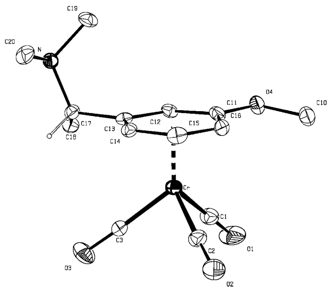
Figure 8. Displacement ellipsoids plot (PLATON) of (S,Sp)-36. Ellipsoids are shown at the 30% probability level. The H-atom attached to the stereogenic centre is shown with arbitrary radius; other H-atoms have been omitted for clarity.
