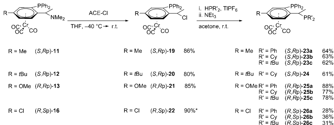
Scheme 7. Yields of isolated products (* yield of crude product) obtained from the nucleophilic replacement of the dimethylamino group by chloride and of diphosphanes prepared by replacement of benzyl chloride with a secondary phosphane HPR'₂. Both reactions take place with retention of configuration.
