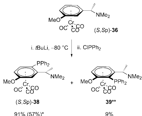
Scheme 15. Lithiation of (S,Sp)\text{-36} and subsequent electrophilic quenching with \text{ClPPh}_2 . * Yield of isolated products. ** The structure of complex 39 is only a proposal.
