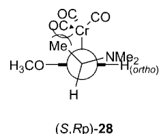
Figure 10. Conformation of (S,Rp)-28 required for ortholithiation assisted by the benzylic dimethylamino group.
