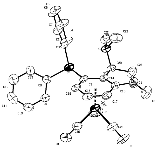
Figure 9. Displacement ellipsoids plot (PLATON) of (S,Sp)-37. Ellipsoids are shown at the 30% probability level. The H-atom attached to the stereogenic centre is shown with arbitrary radius; other H-atoms have been omitted for clarity.
