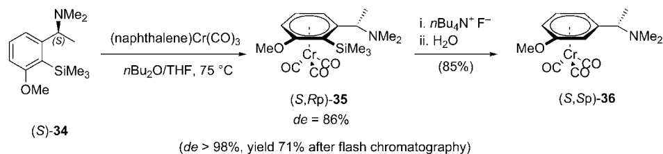
Scheme 13. Stereoselective route to (S,Sp)-36.
