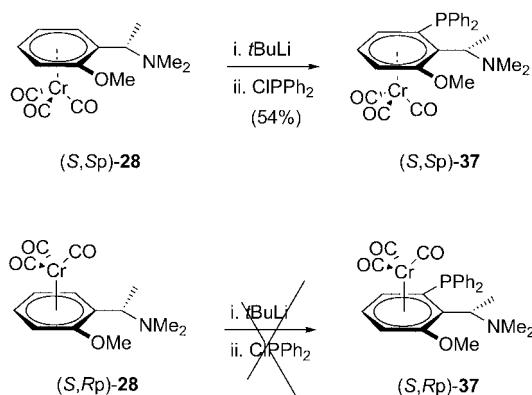
Scheme 14. Lithiation of diastereomeric complexes (S,Sp)-28 and (S,Rp)-28 and subsequent electrophilic quenching with \text{ClPPh}_2 . The latter complex fails to react (see text for experimental conditions).
