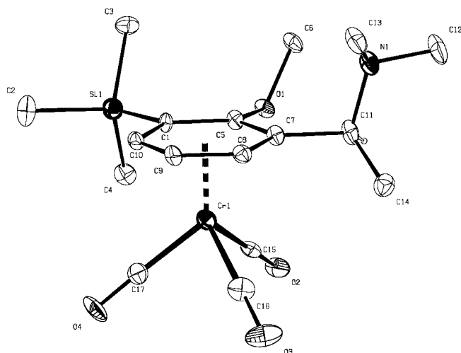
Figure 6. Displacement ellipsoids plot (PLATON) of one independent molecule of ( S,Rp )- 30 . Ellipsoids are shown at the 30% probability level. The H-atom attached to the stereogenic centre is shown with arbitrary radius; other H-atoms have been omitted for clarity.
