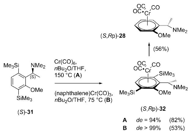
Scheme 10. Stereoselective route to ( S,Rp )- 28 .
