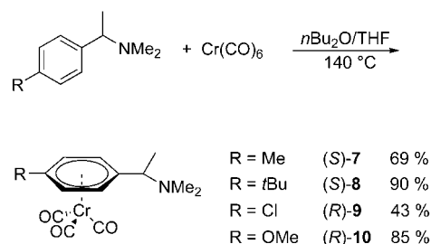
Scheme 3. Yields obtained in the complexation of protected para -substituted benzylamines with \text{Cr}(\text{CO})_6 .
