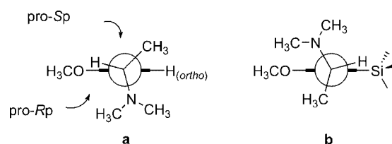
Figure 5. (a) Preferred average conformation adopted by ( S )- 4 in solution at room temperature as inferred by difference NOE/ 1 H NMR experiments. (b) Preferred conformation in the presence of a bulky –SiMe 3 group in the ortho position.
