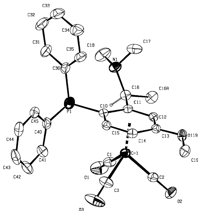
Figure 11. Displacement ellipsoids plot (PLATON) of one independent molecule of (S,Sp)\text{-38} . Ellipsoids are shown at the 30% probability level. The H-atom attached to the stereogenic centre is shown with arbitrary radius; other H-atoms have been omitted for clarity.
