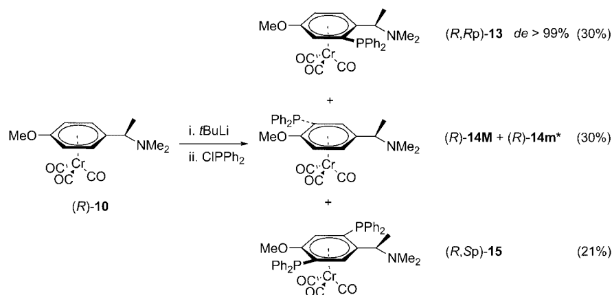
Scheme 5. Products obtained in the ortho -functionalisation of ( R )- 10 . Yields of isolated products are reported in parentheses. * This notation indicates the two regioisomeric products bearing a diphenylphosphanyl group ortho to the OMe substituent; the absolute configurations, however, could not be assigned.
