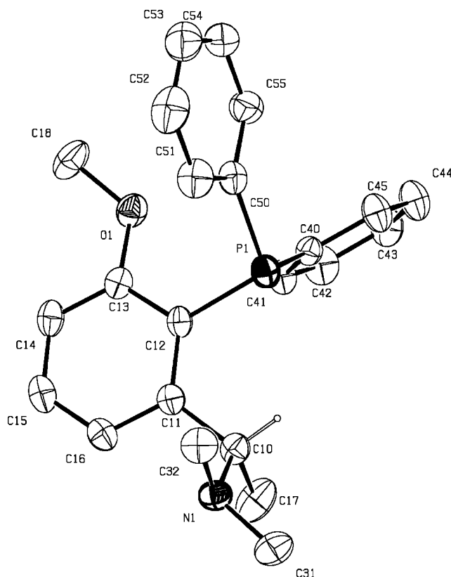
Figure 7. Displacement ellipsoids plot (PLATON) of one independent molecule of ( S )- 33 . Ellipsoids are shown at the 30% probability level. The H-atom attached to the stereogenic centre is shown with arbitrary radius; other H-atoms have been omitted for clarity.
