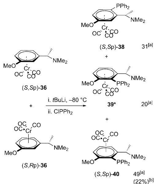
Scheme 16. Products arising from ortho -functionalisation of a 1:1 diastereomeric mixture of (S,Sp)\text{-36} and (S,Rp)\text{-36} . * The structure of complex 39 is only a proposal. [a] Relative amounts of products as inferred from the ^{31}\text{P} NMR spectrum of the crude reaction mixture. [b] Yield after flash chromatography; only this product was isolated.
